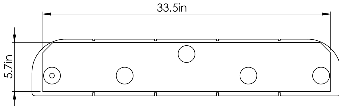
BOTTOM GLUE DOWN PLATE SIZE REQUIRES 1/6 QUART OF EPOXY
