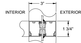
VIEW C-C
