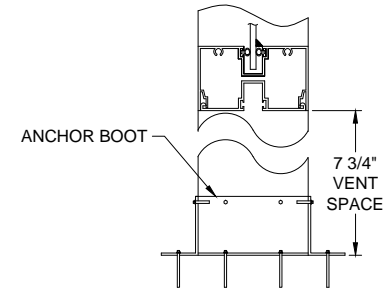
VIEW D-D
