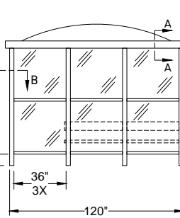
ELEVATION C
