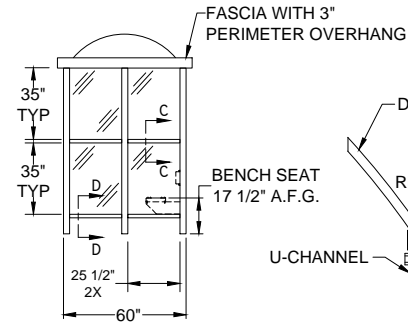
ELEVATION D
