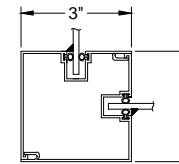
VIEW B-B
