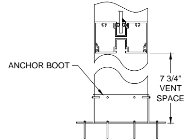
VIEW D-D
