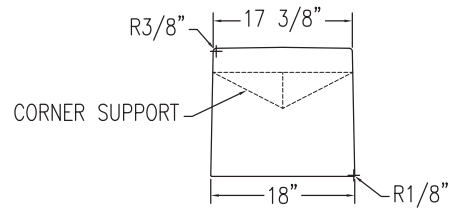
4 END VIEW Scale: 1/16" = 1"
