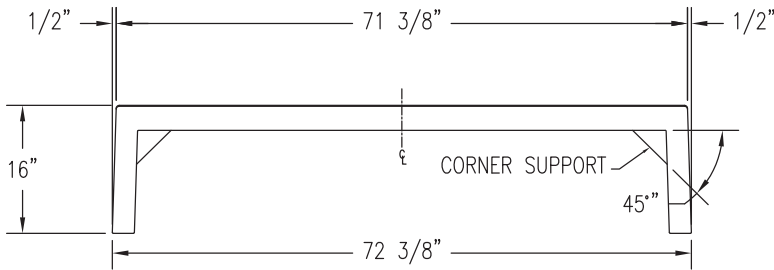
2 ELEVATION VIEW Scale: 1/16" = 1"
