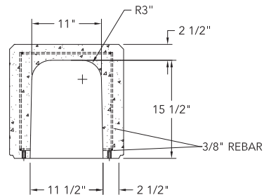
5 SECTION VIEW
