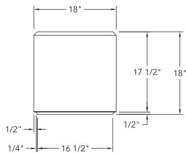
4 END VIEW
