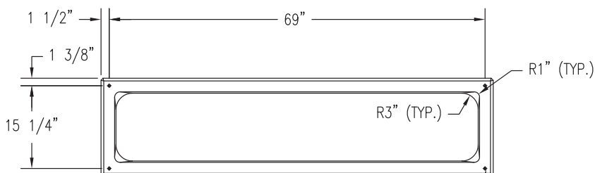
4 BOTTOM VIEW Scale: 1/16" = 1"
