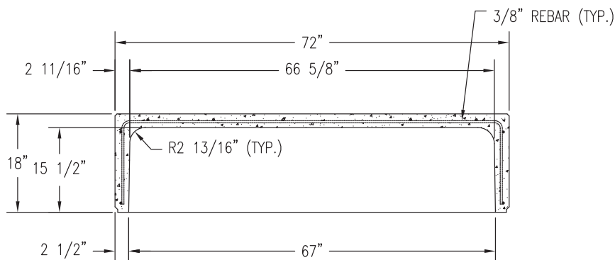
3 SECTION VIEW Scale: 1/16" = 1"
