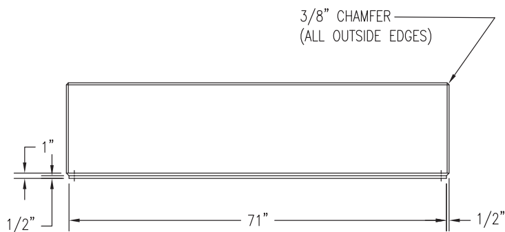
2 ELEVATION VIEW Scale: 1/16" = 1"
