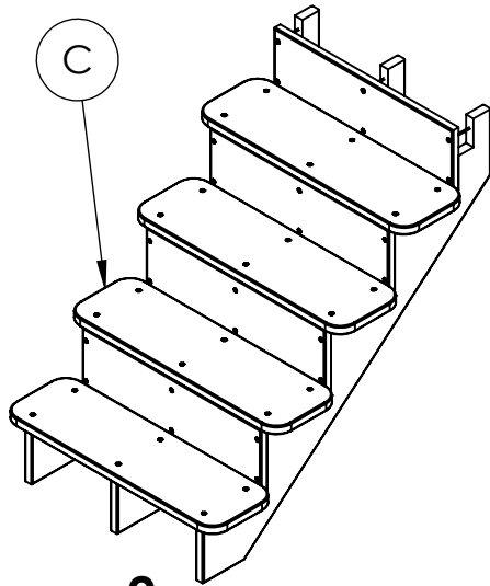
2 STAIR ASSEMBLY
